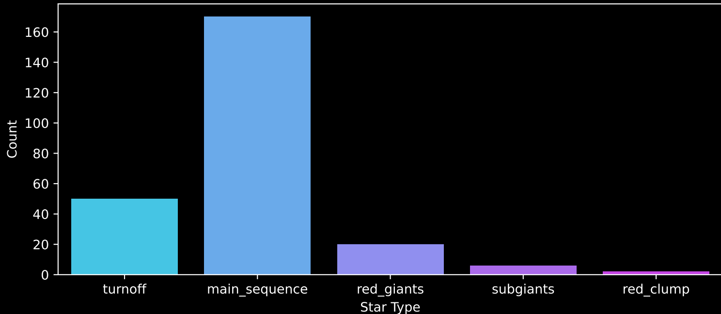
GALAH DR4 Field: [7032] Count plot of Star Type
