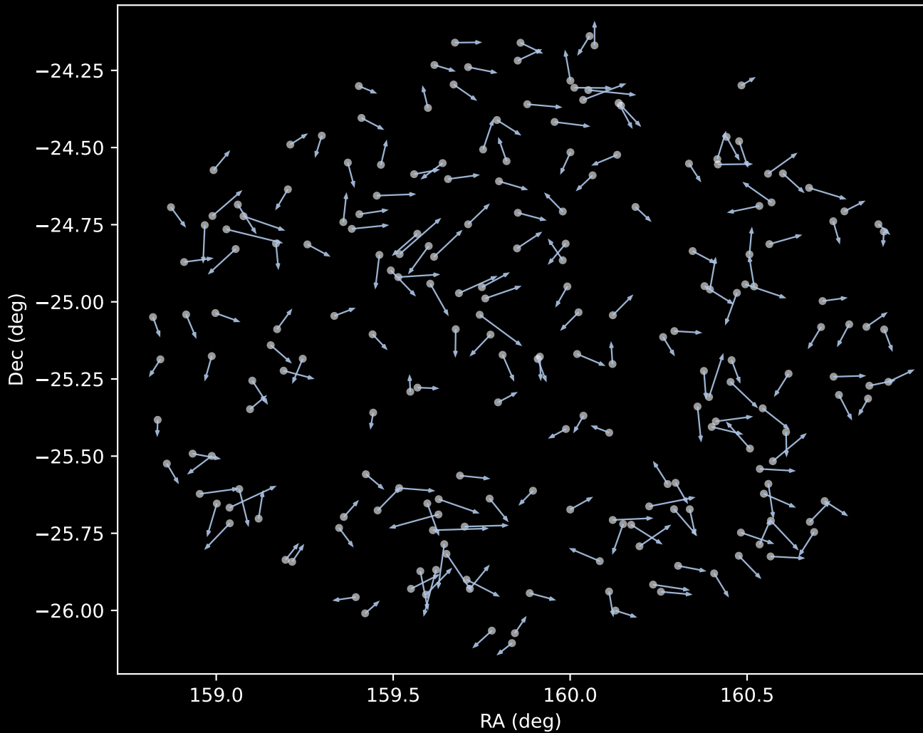
GALAH DR4 Cluster 1 Proper Motion Vectors (n=212)
