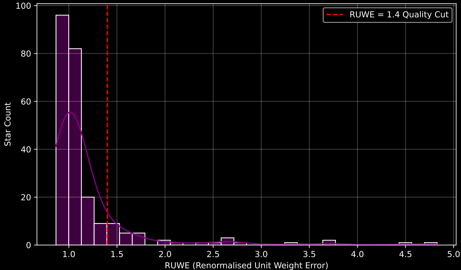
GALAH DR4 Field [7032] RUWE Distribution (n= 240)
