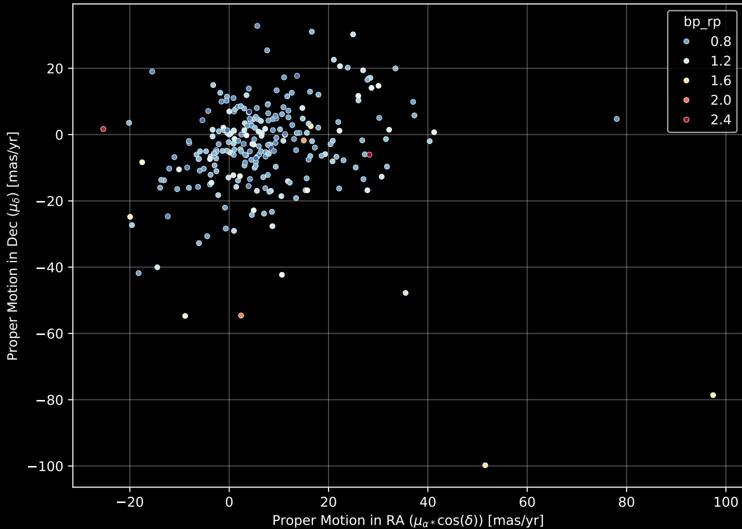
GALAH DR4 Field: [7032] Proper Motion Diagram (n= 248)
