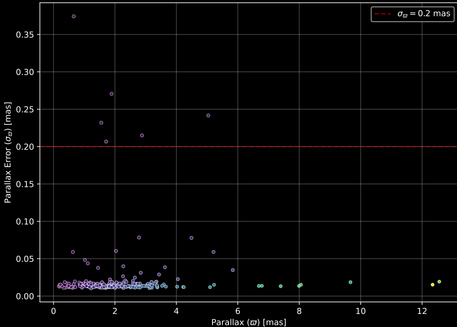
GALAH DR4 Field: [7032] Parallax Quality (n= 248)
