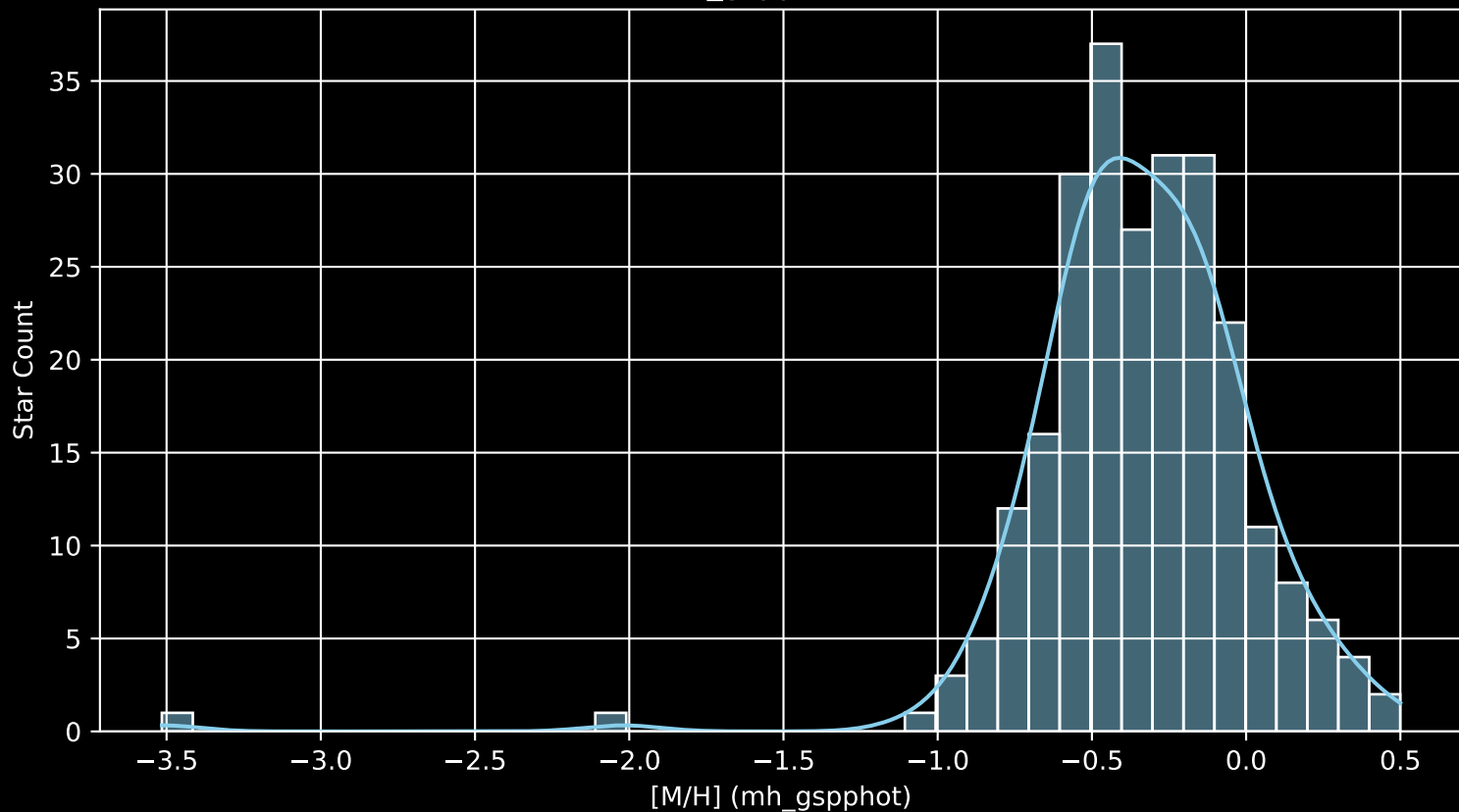
GALAH DR4 Field: [7032] [M/H] (mh_gspphot) (n= 248)
